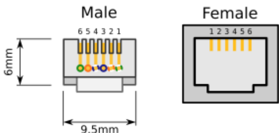
6P6C - RJ12 (RJ25)
